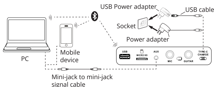
Fig.3. Connection diagram
